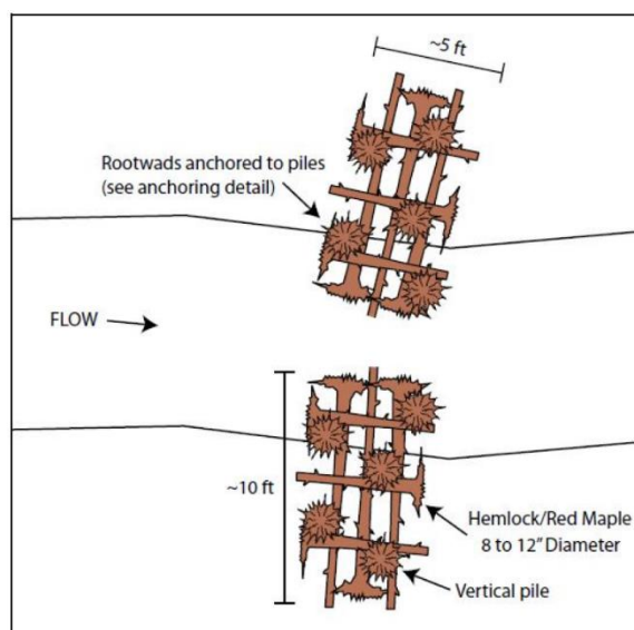
Concept plan for Barberry Creek log constrictors
